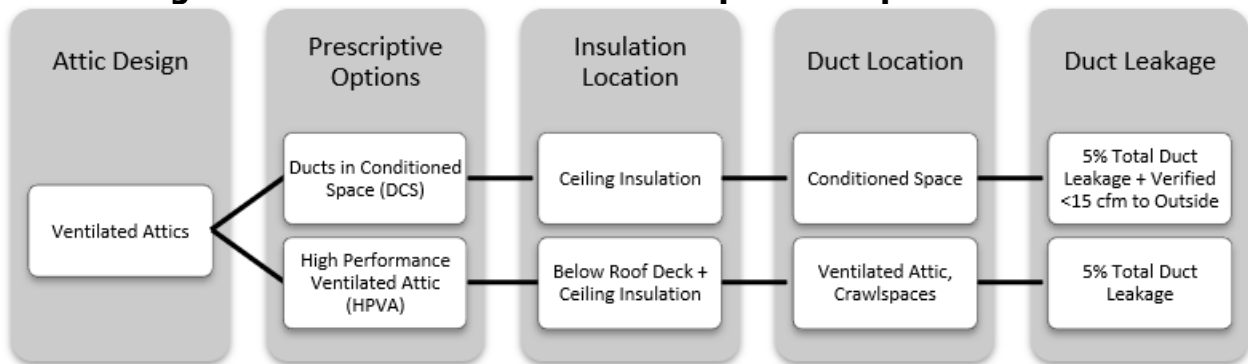
Figure 3-22: Ventilating Attic Prescriptive Compliance Choices
