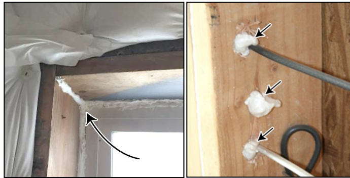
Figure 3-10: Air Sealing
